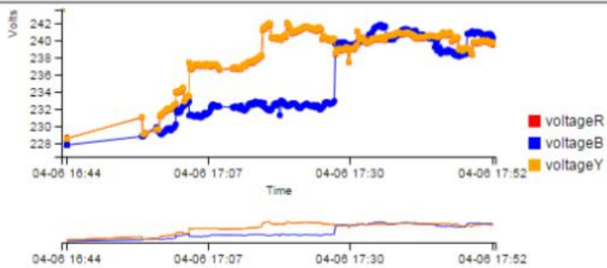
Voltage Chart
